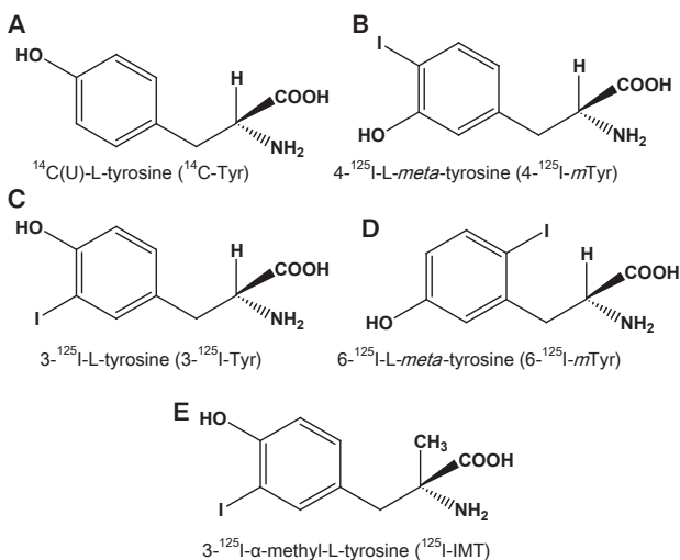
Fig. 1 Chemical structures of L- 14 C(U)-Tyr (A), 4- 125 I-L- meta -tyrosine (4- 125 I- m Tyr) (B), 3- 125 I-L-tyrosine (3- 125 I-Tyr) (C), 6- 125 I-L- meta -tyrosine (6- 125 I- m Tyr) (D) and 3- 125 I-iodo- \alpha -methyl-L-tyrosine ( 125 I-IMT) (E).
